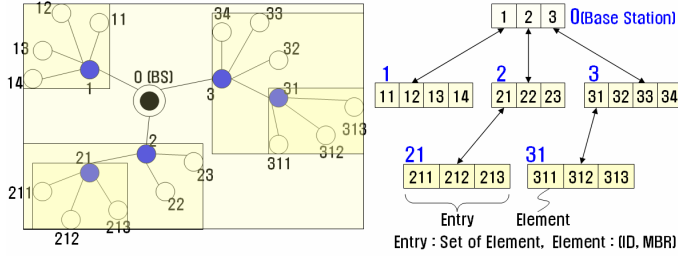
Fig. 4. A GRT Example. Gray circles mean intermediate parent nodes.
