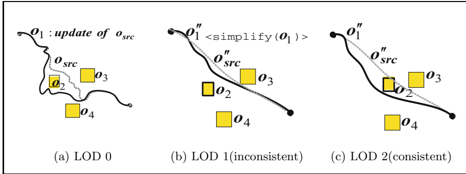
Fig. 3. Directional Consistency for Line-Simplification
