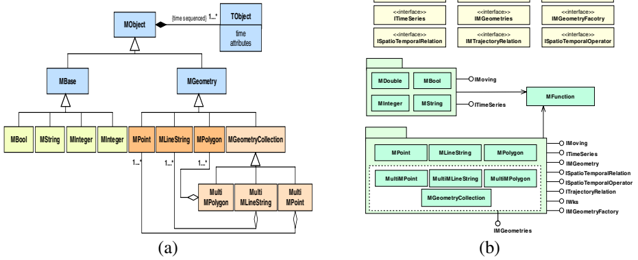
Fig. 2. Moving Objects Data Types : (a) Moving Objects Class Hierarchy (b) Interface Diagram of Moving Objects Component
