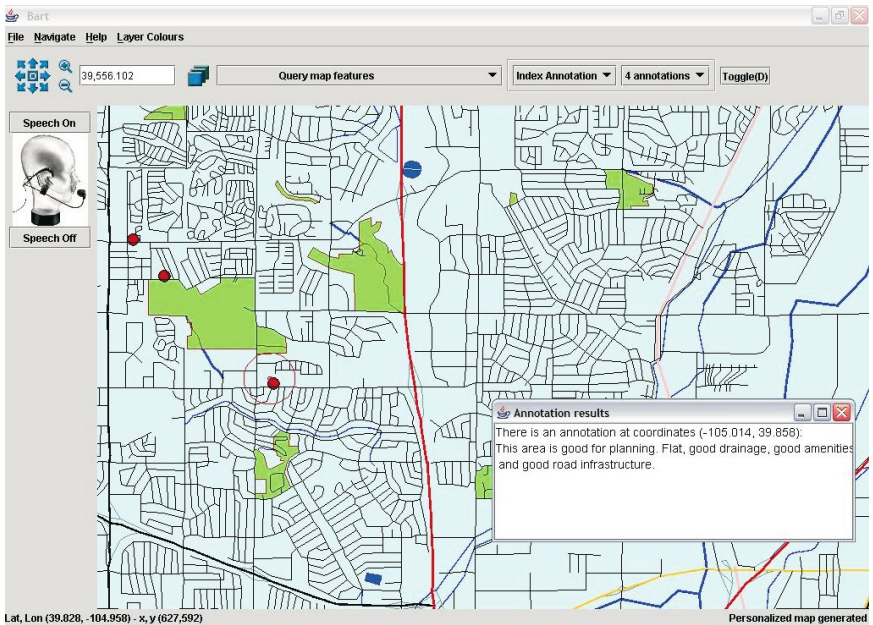
Fig. 2. CoPASS ScreenShot
