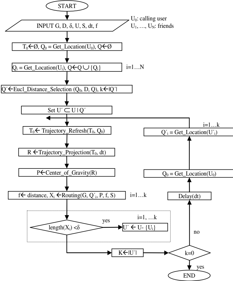
Fig. 6. Get-together algorithm
