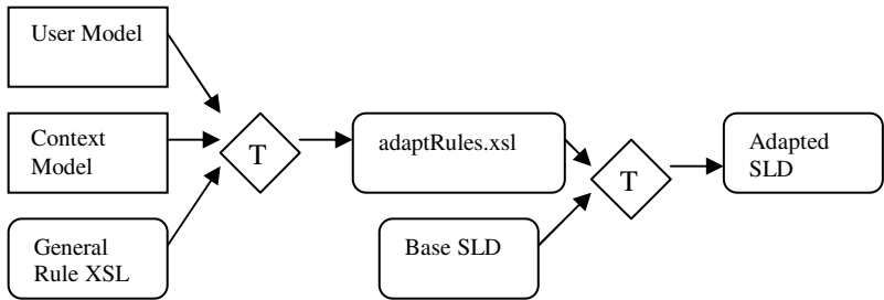
Fig. 6. Extension of the transformation cascade in order to generated an adapted SLD from User and Context Models and general rules how to apply these (specified in XSL)
