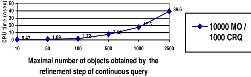
Fig. 12. The average CPU time needed for data structures update upon location/speed update of a mobile object
