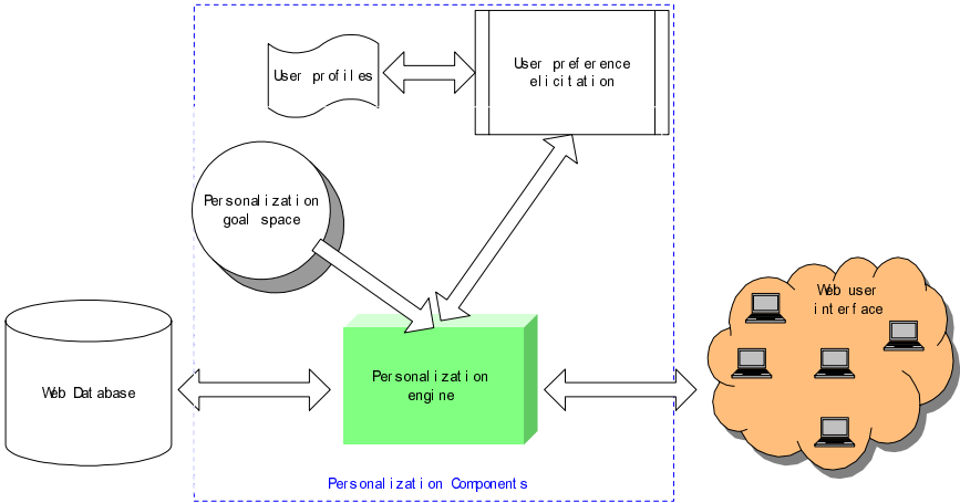
Fig. 1. Personalization components
